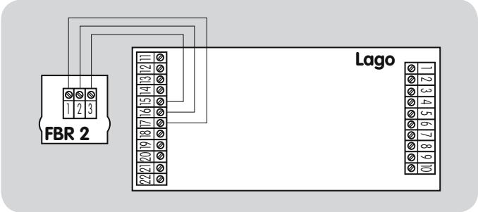
FBR 2 with Lago 0321 and Lago 0101/1001
