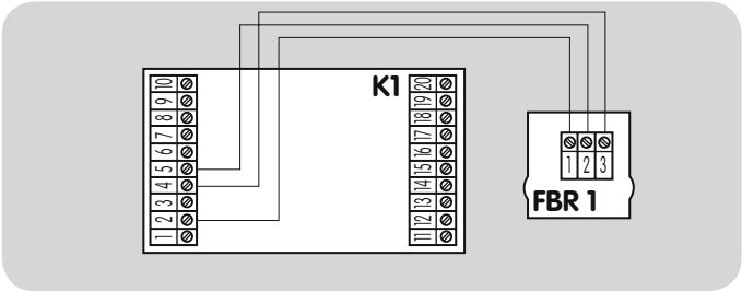
FBR 1 with E25
